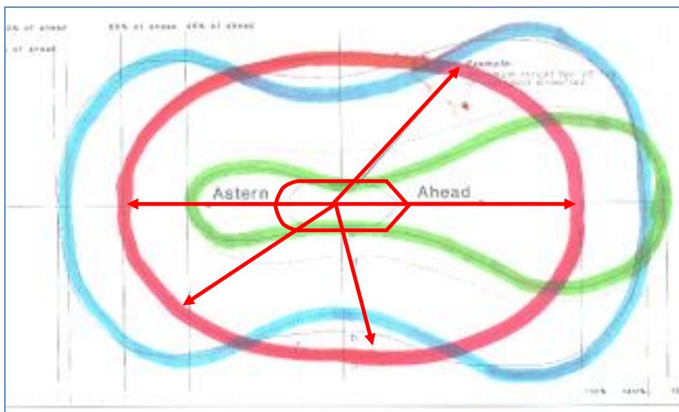
Fig. 10 Bollard pull vector diagram for various types of propulsion
