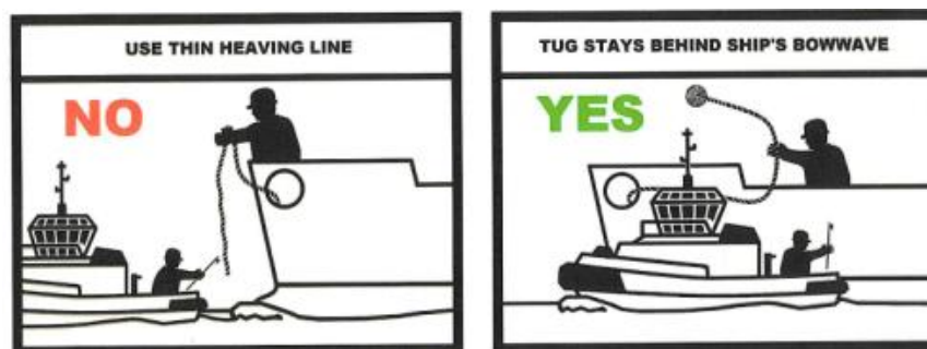
Fig. 18 Pass the heaving line from the ship's shoulder
