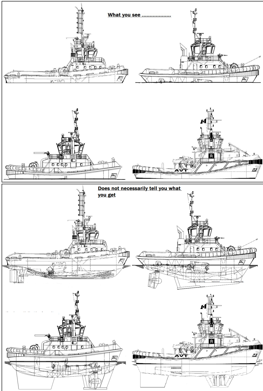
Fig. 2 Different types of hull design and propulsion
