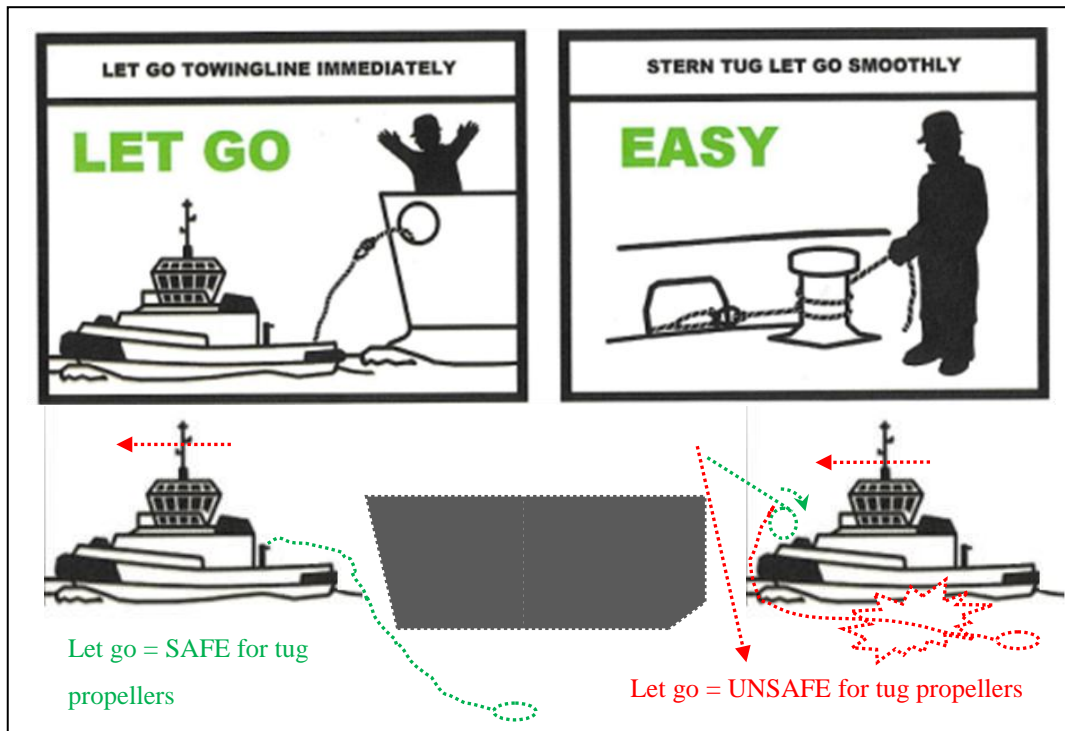
Fig. 22 Releasing tugs - different procedure for bow and stern tug
