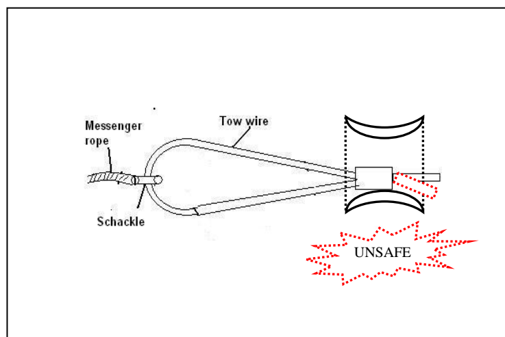
Fig. 28 Risk of towline parting when clamp rests against fairlead
