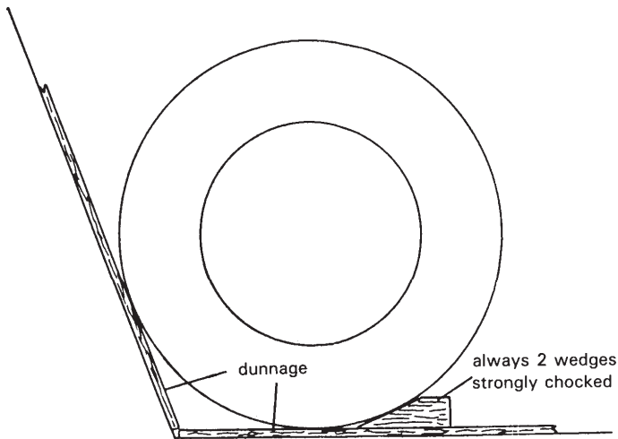
Figure 1 - Principle of dunnaging and wedging coils
