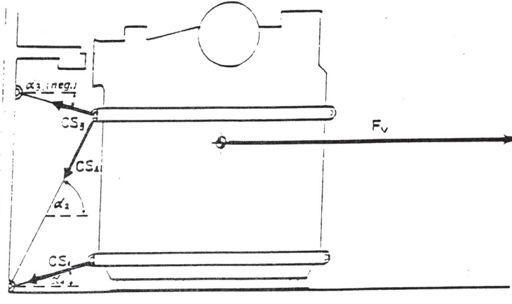
Figure 1: Balance of transverse forces
