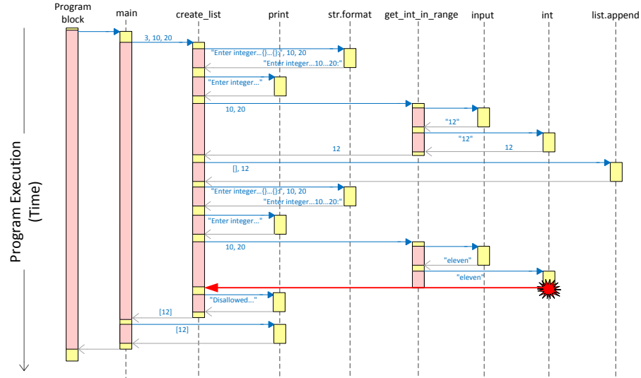
Figure 12.4 The execution sequence of a sample run of Listing 12.13 (makeintegerlist2.py) in which the create_list function handles the exception. Observe that the int function does not return to get_int_in_range as it normally would, but rather int bypasses get_int_in_range on its way to the nearest exception handler, which it locates in create_list.
