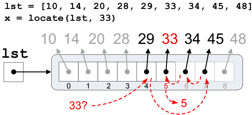
Figure 15.4 Binary search begins in the middle of an ordered list. The algorithm jumps forward or backward as needed in decreasing stride amounts. Each successive probe reduces the number of elements in its search space by one-half.
